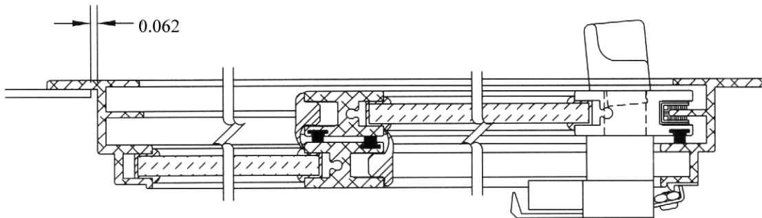
SECTION A-A FLANGE MOUNT
