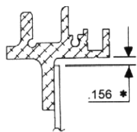
FLANGE MOUNT
