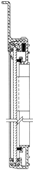
SECTION A-A (WITH WIPER PLATE)
